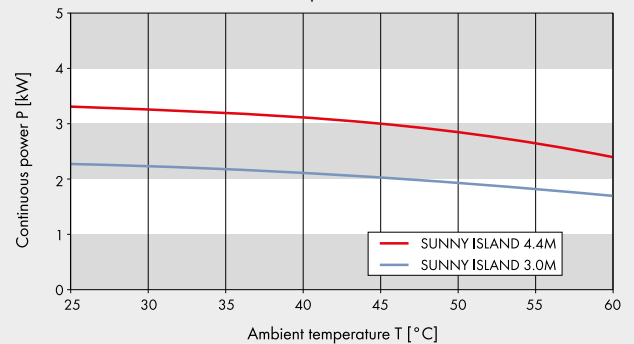
Power-temperature curve
