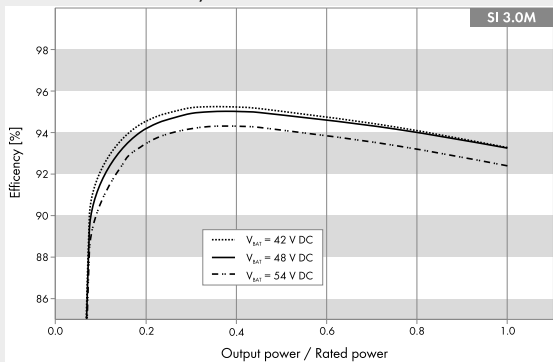
Efficiency curve SUNNY ISLAND 3.0M
