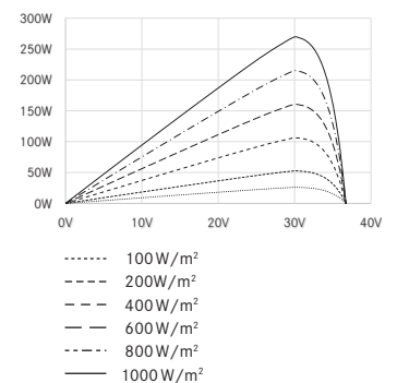
UP-Kennlinie Bsp. LX-270P/156-60+
